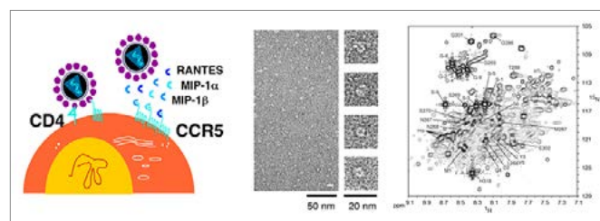
Left: docking of HIV-1 to the receptors CD4 and CCR5 on T-cell surface. Middle: electron micrograph showing detergent micelles containing CCR5. Right: ^1\text{H} - ^{15}\text{N} spectrum of CCR5 in detergent micelles.
