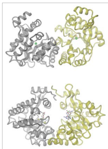
Close-up of the EAL dimer of YahA ( E. coli ) induced by binding of c-di-GMP. Adopted from Sundriyal et al. , 2014.
