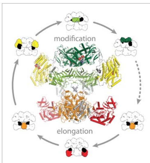
Fig. 3: Hybrid highresolution structure of a fully-reducing iterative polyketide synthase (Herbst et al. , Nature, 2016).
