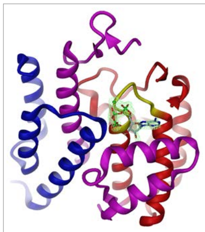
Crystal structure of Fic protein VbhT in complex with anti-toxin VbhA (blue). Also shown is the ATP substrate (with electron density). Adopted from Engel et al. , 2012.
