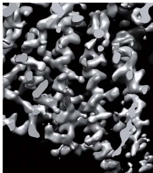
C-CINA: Cryo-EM of biological molecules can reach atomic resolution. Here, details from the type-6-secretion system show alpha-helical structures.
